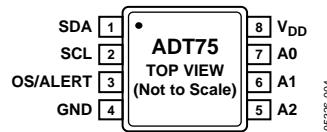
Figure 4. LFCSP Pin Configuration
