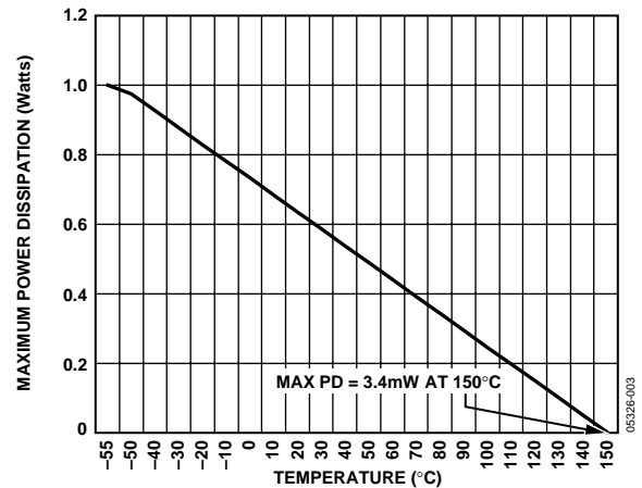
Figure 3. MSOP Maximum Power Dissipation vs. Temperature
