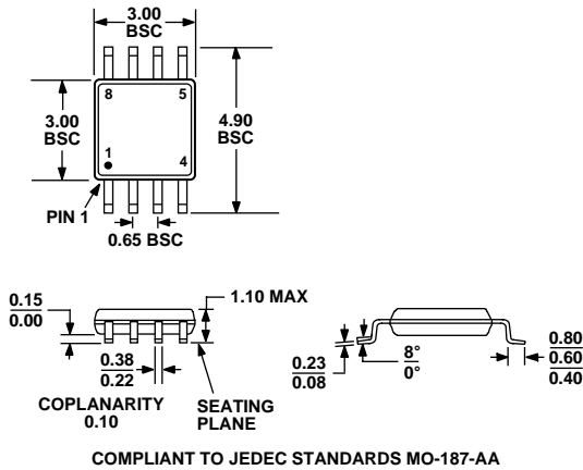
Figure 23. 8-Lead Mini Small Outline Package [MSOP] (RM-8) Dimensions shown in millimeters
